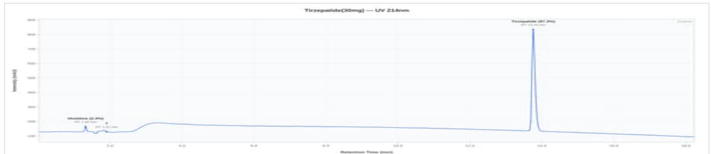
Tirzepatide 30mg - LOT - TR - QSCT1: UV Chromatogram
